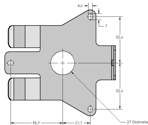
Figure 4 – Mounting Plate Hole Dimensions (mm)
