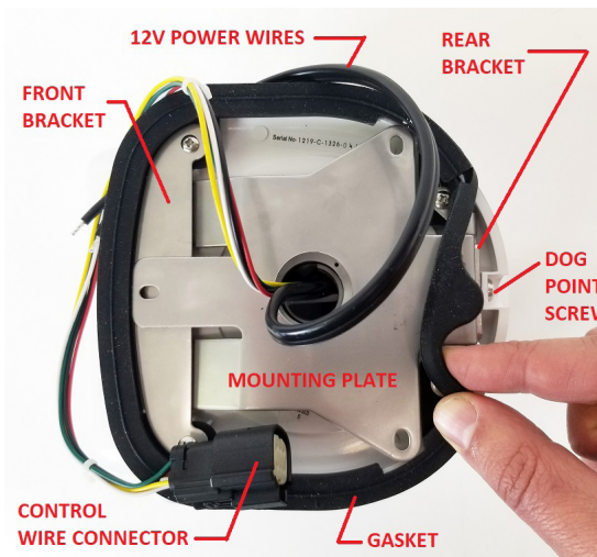
Figure 3 – Stryker® ST viewed from bottom
