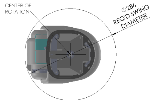
Figure 2 – Permanent Mount Stryker® ST Spotlight – Bottom View Looking Up -Dimension in mm
